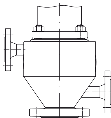
Heating jacket
