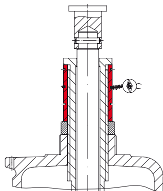
Lock bushing
